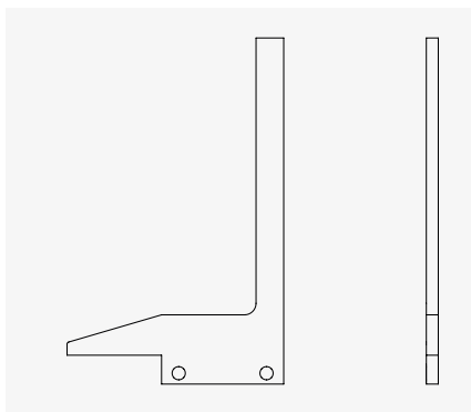
TRIANGULAR PUSHER
