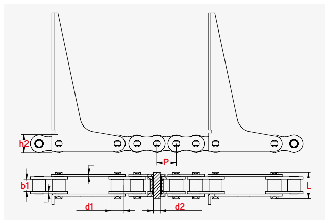
BENT PUSHER
